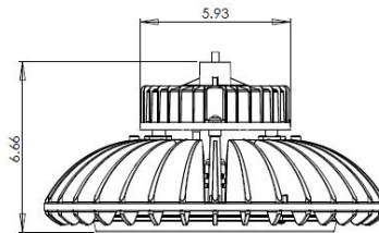
18000L Model
