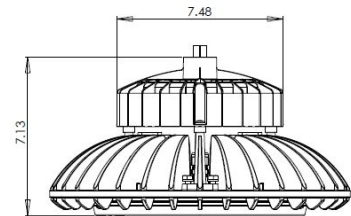
24000L Model
